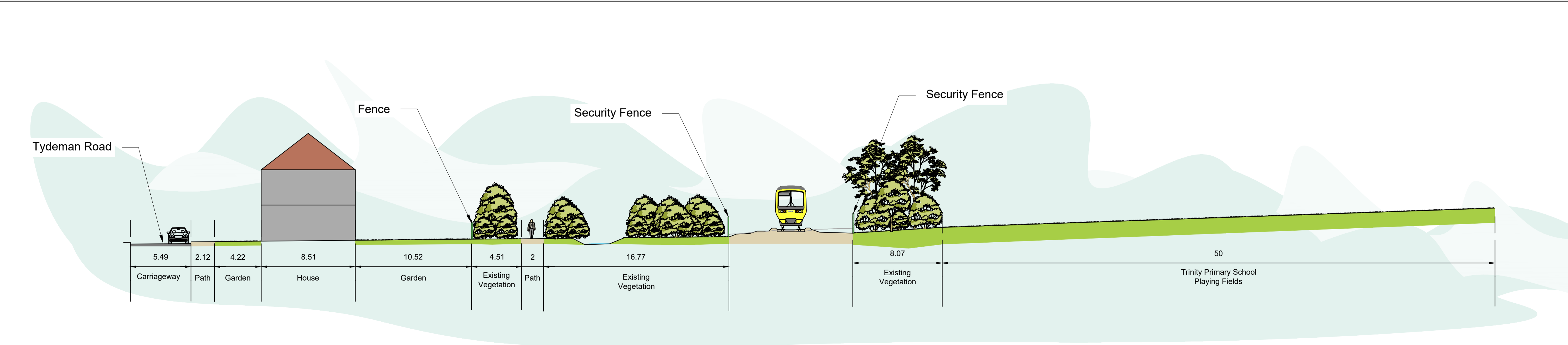
Section CC
