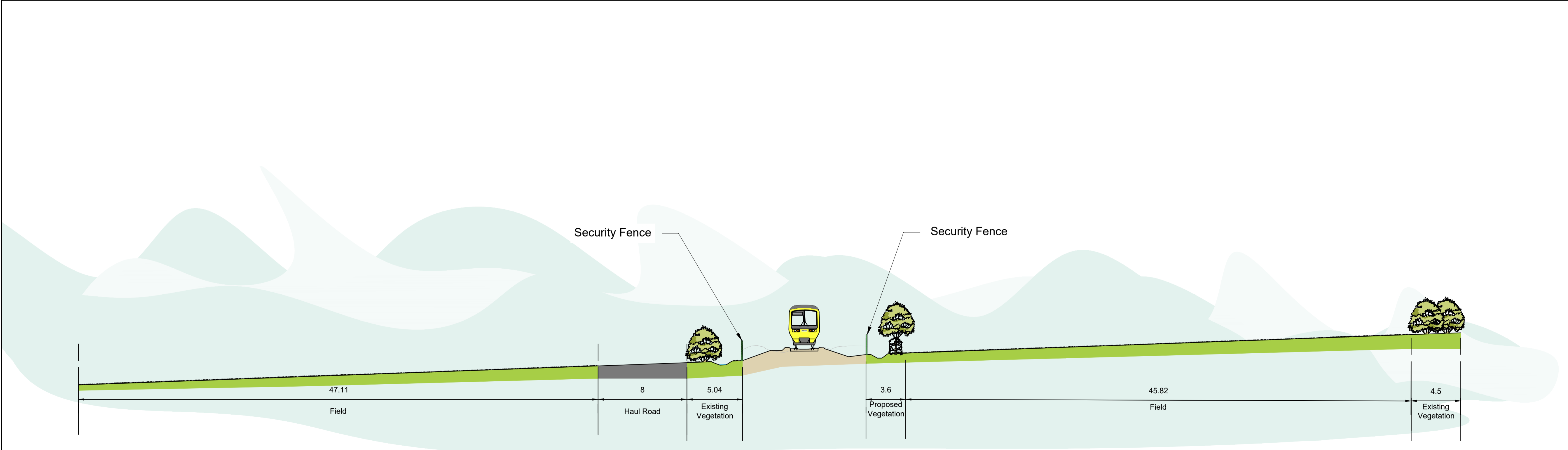
Section EE
